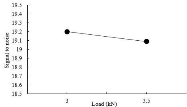
Fig. 11 Signal to noise ratio of load parameter
