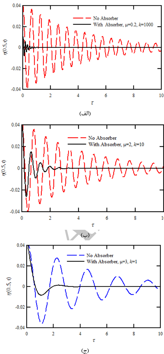
Fig. 4. Influence of the vibration absorber on the dynamic response of the fluid conveying pipe for different values of the fluid velocity, (a) u = 0.2 , (b) u = 2 , and (c) u = 3
