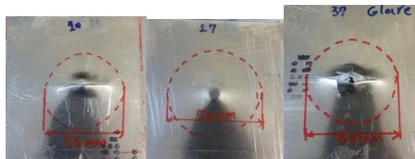
Fig. 13 Damage zone propagation on target No.10 (hemispherical projectile), No.27 (flat projectile) and No.37 (conical 90° projectile)
