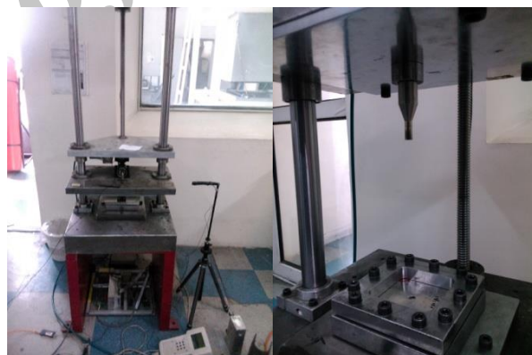
Fig. 5 Drop weight testing machine
