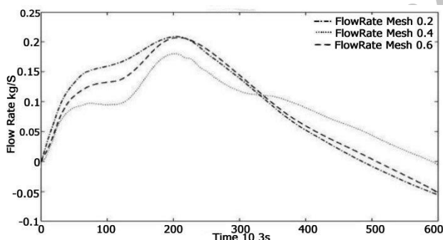
Fig. 10 Mass flow rate in worst case design
