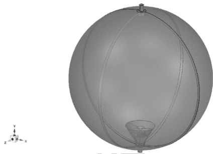
Fig. 15 Final tank and PMD schematic
