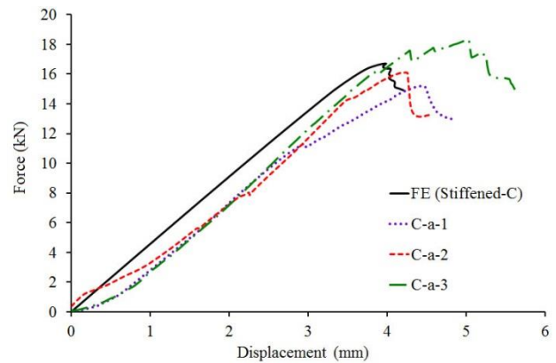
Fig. 11 The force-displacement diagram for stiffened shell type C
