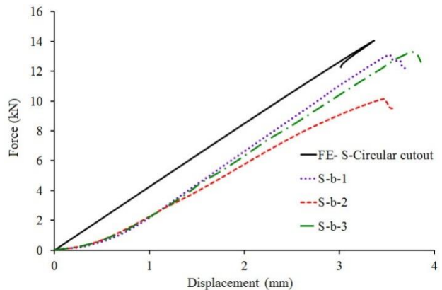
Fig. 14 The force-displacement diagram for unstiffened shell with opening
