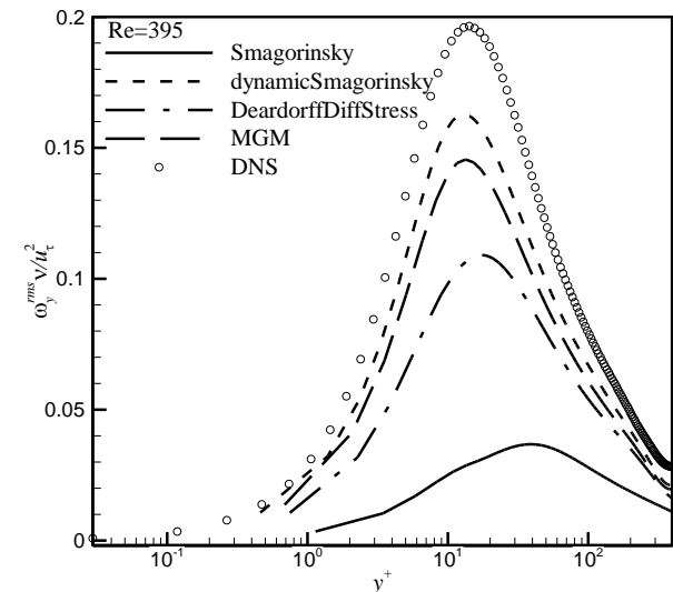
Fig. 9 Profiles of the normalized standard deviation of the wall-normal component of vorticity, \omega_y^{rms} v / u_\tau^2
