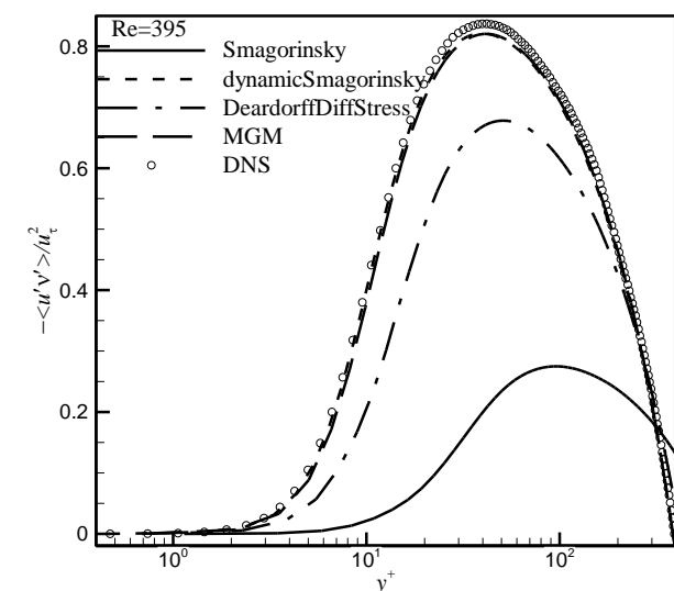
Fig. 7 Profiles of the normalized turbulent shear stress, -\langle u'v' \rangle / u_\tau^2
