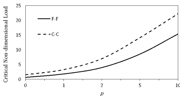
Fig. 7 Effects of combination of the functionally graded material cylindrical shell supported on critical buckling pressure for different boundary conditions
