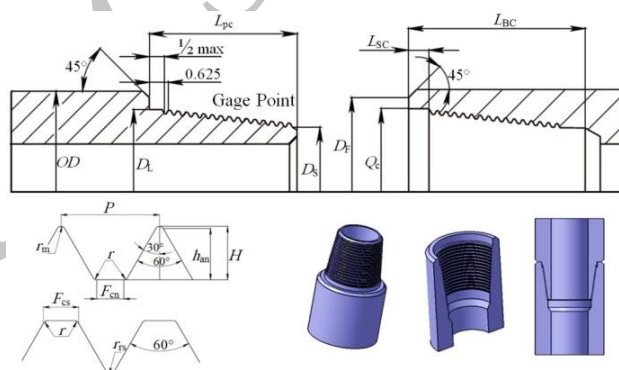
Fig. 6 Specification and geometry shape of API NC46 tool joint
