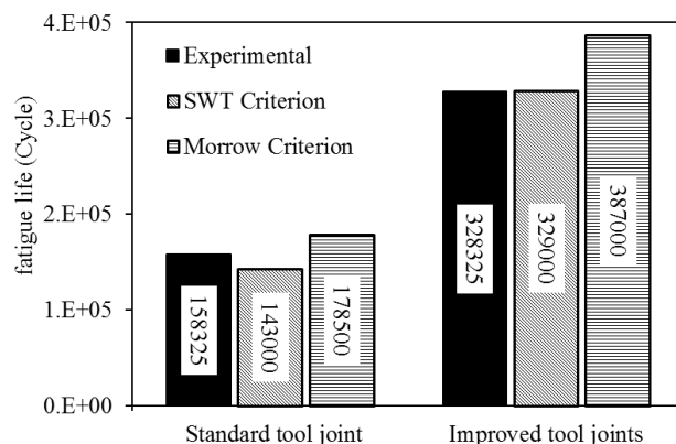
Fig. 20 Fatigue life comparison between improved and standard tool joints
