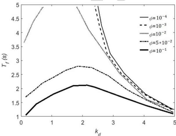
Fig. 20 Preferred regions of T_f versus k_d for different values of \phi = 10^{-4}, 10^{-3}, 10^{-2}, 5 \cdot 10^{-2}, 10^{-1} ( u_{on} = 0.3, h = 0.15 )
