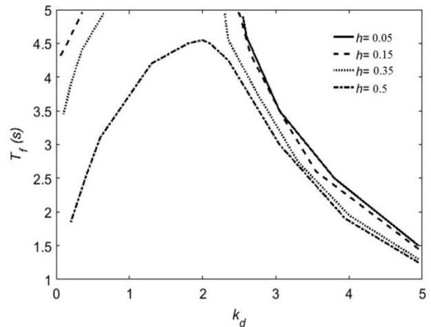
Fig. 21 Preferred regions of T_f versus k_d for different values of h = 0.05, 0.15, 0.35, 0.5 ( u_{on} = 0.5, \phi = 10^{-2} )
