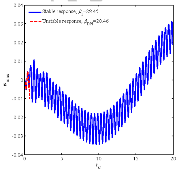
Fig. 4 Damped stable and unstable time response of the micro-gyroscope for (a) drive direction and (b) sense direction
