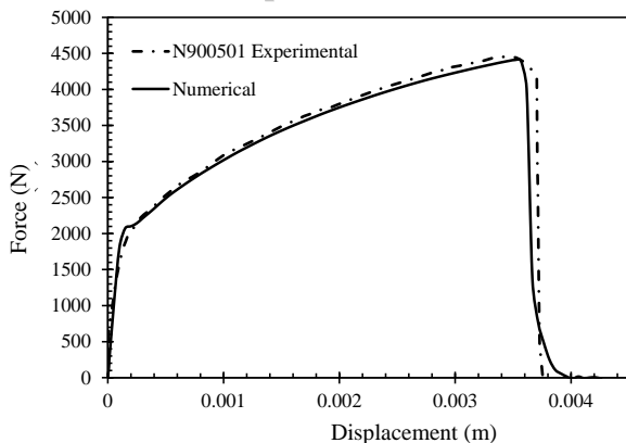
Fig. 11 Force-Displacement response of 5 mm notched specimen
