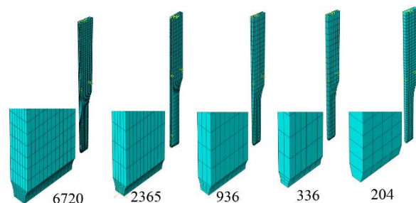
Fig. 8 Mesh Convergence Analysis
