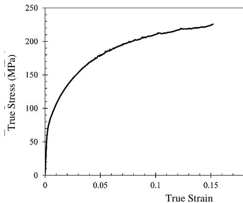
Fig. 5 True Stress-Strain Curve of AL2024-O
