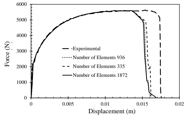
Fig. 6 Force-Displacement of Flat Specimen
