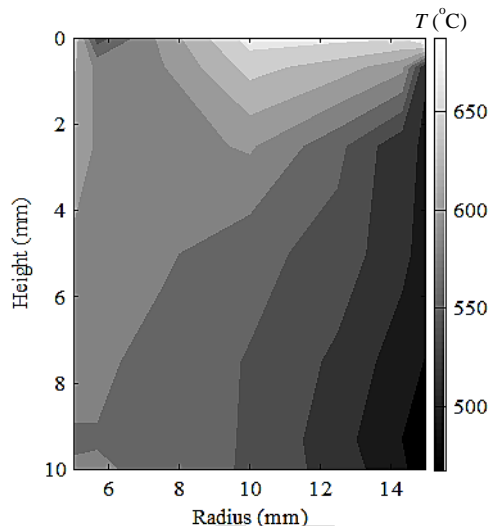
Fig. 6 Temperature distribution (°C) in section 2 of aluminum workpiece
