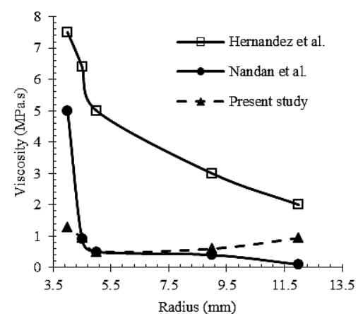
Fig. 13 Viscosity distribution in section 3 of steel workpiece under the shoulder ( z=0 ).
