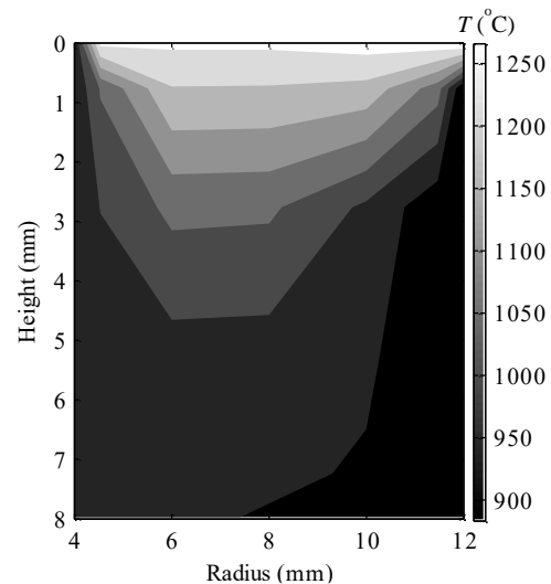
Fig. 12 Temperature distribution (°C) in section 2 of steel workpiece
