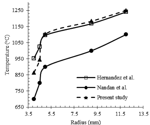
Fig. 11 Temperature distribution (°C) in section 3 of steel workpiece under the shoulder.
