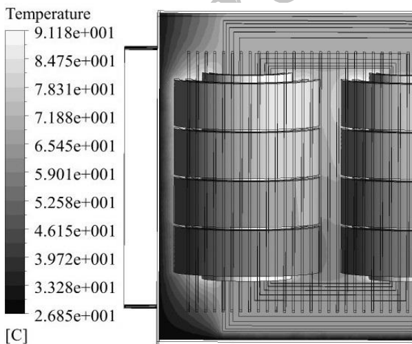
Fig. 21 Temperature distribution external view in silicon core transformer in full load conditions
