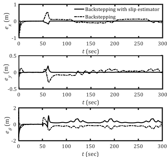
Fig. 6 Error signals of tracking control
