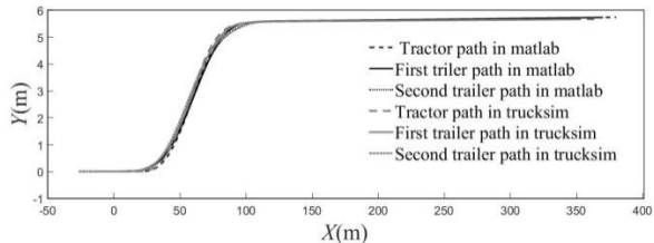
Fig. 18 Lane change paths of vehicle with new controller
