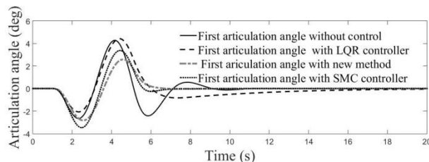
Fig. 21 Changes in first articulation angle with various controllers
