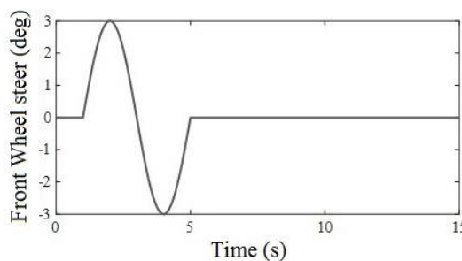
Fig. 5 Steering Angle
