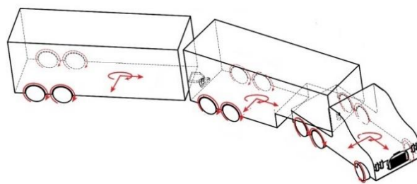
Fig. 1 Multi trailer articulated vehicle
