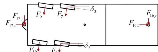
Fig. 3 The forces enter first trailer
