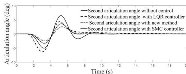
Fig. 22 Changes in second articulation angle with various controllers
