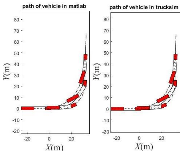
Fig. 23 Paths of vehicle with LQR controller
