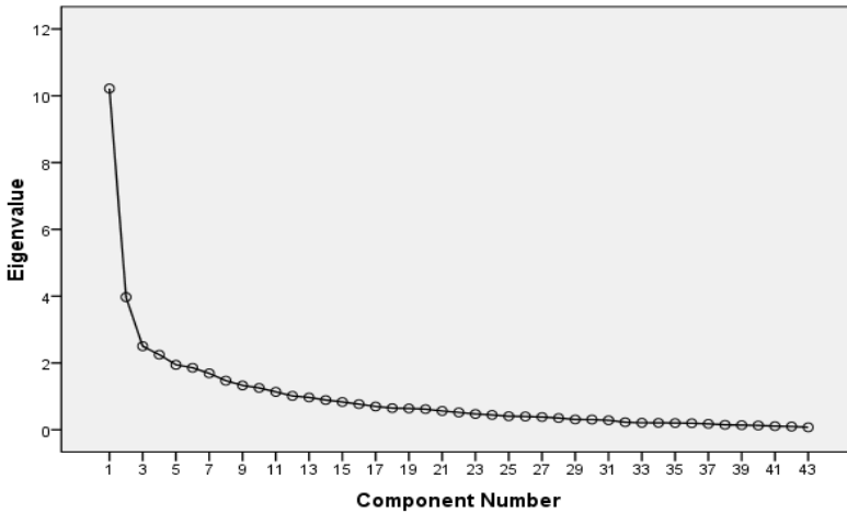
Scree Plot
