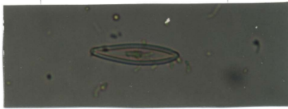
Gomphonema
