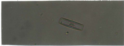
Diatoma
