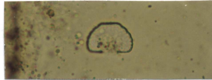
Cosmarium
