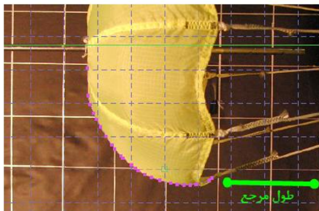
Fig. 2. Profile extraction of inflated canopy
