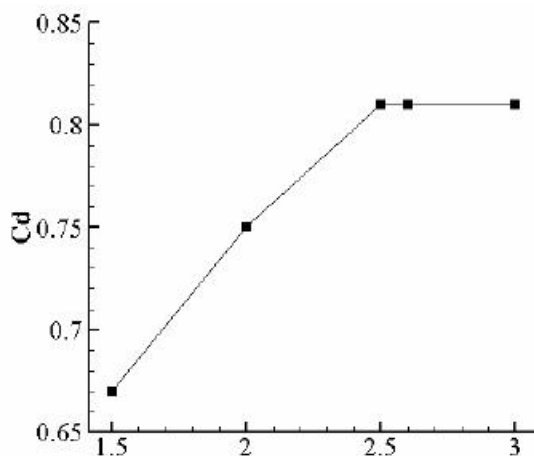
Fig. 4. Mesh independency
