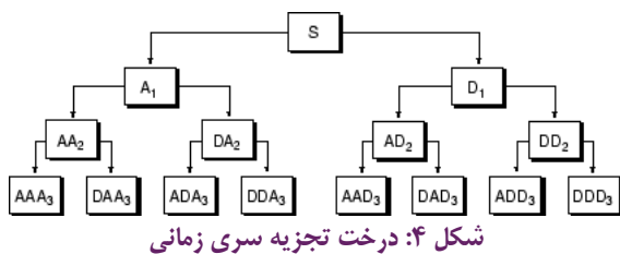
Fig.4. Decomposition tree of time series
