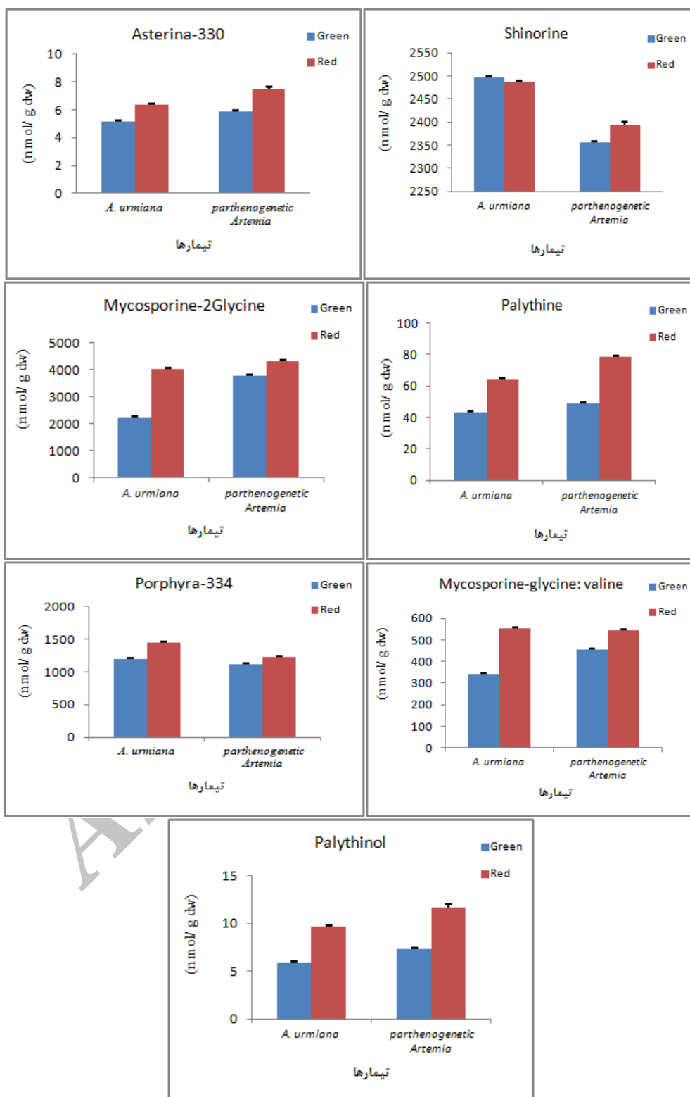
( ) MAs Dunaliella salina ( ) parthenogenetic Artemia A. urmiana ( )
