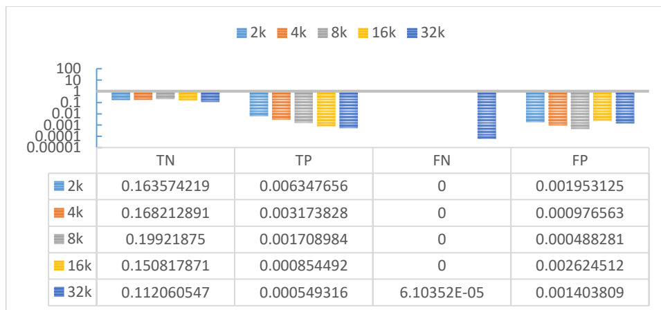
(شکل-7): نمودار لگاریتمی نسبت (False Negative (FN), False Positive (FP), True Negative (TN) and True Positive (TP) (Figure-7): The logarithmic rates of False Negative (FN), False Positive (FP), True Negative (TN) and True Positive (TP)
