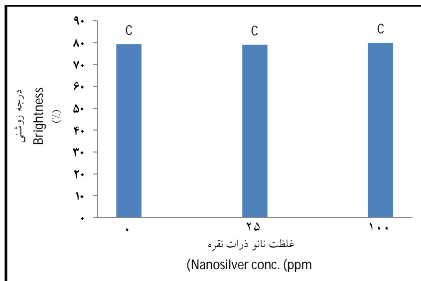
Figure 9- The effect of using Nanosilver on paper brightness.
