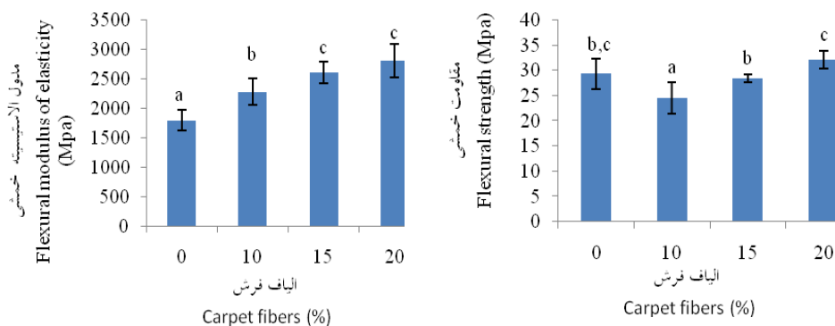
Figure 3. Effect of waste carpet fibers on the flexural modulus of elasticity and flexural strength.
