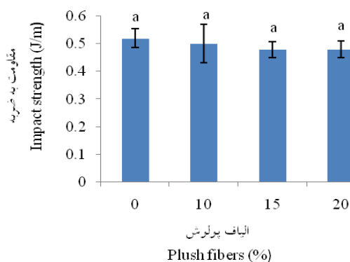
Figure 5. Effect of waste plush fibers on impact strength.
