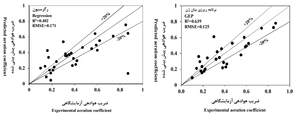
Figure 1. Relation between experimental and predicted data of aeration coefficient (β) at training and testing stages using GEP and regression models.
