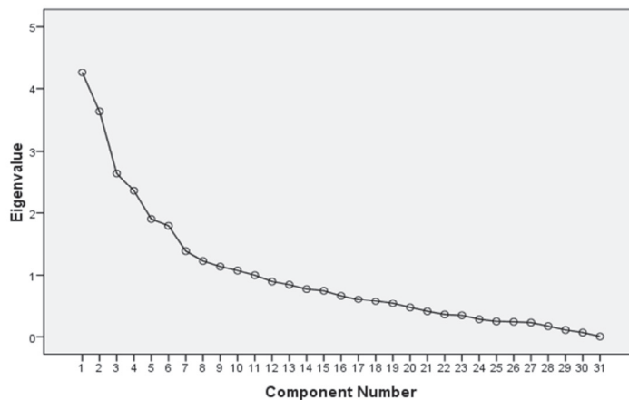
Scree Plot
