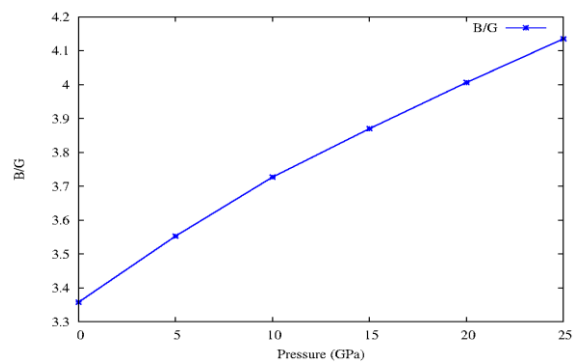
Figure 8. B/G ratio of TiPdSn in cubic phase.
