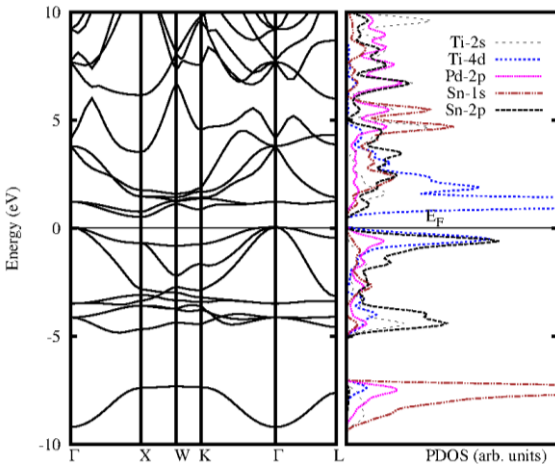
Figure 4. Electronic band structure and DOS of TiPdSn in cubic phase at zero pressure.
