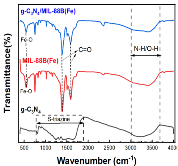
Figure 2. FTIR spectrum of g-C_3N_4 , MIL-88B(Fe), and g-C_3N_4 /MIL-88B(Fe).
