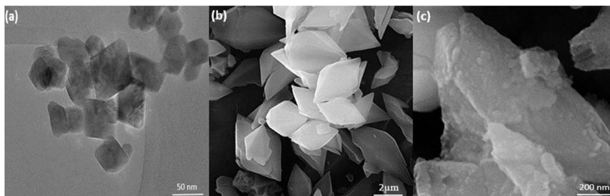
Figure 1. TEM image of (a) g-C_3N_4 , SE micrographs of (b) pure MIL-88B(Fe) and (c) g-C_3N_4 /MIL-88B(Fe) nanocomposite.
