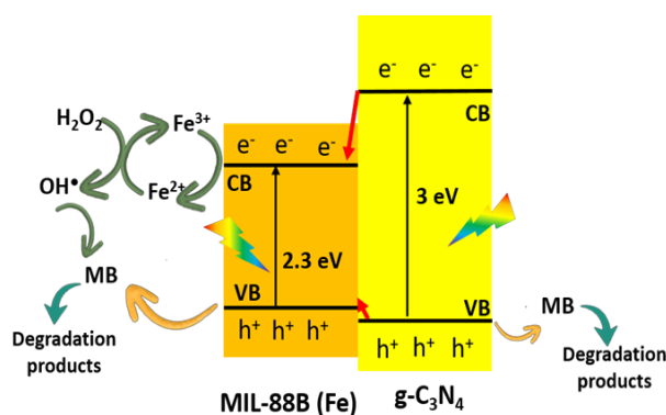
Scheme 1. Proposed mechanism of electron-hole generation, and transfer at the interface of g-C 3 N 4 and MIL-88B(Fe) under UV-Vis. light illumination, and the following photo-Fenton reactions at the surface of g-C 3 N 4 /MIL-88B(Fe) nanocomposite to degrade MB pollutant. (CB MIL-88B(Fe) =-1.55 eV, VB MIL-88B(Fe) =0.73 eV, CB g-C 3 N 4 =-2.2 eV, VB g-C 3 N 4 =0.8 eV).
