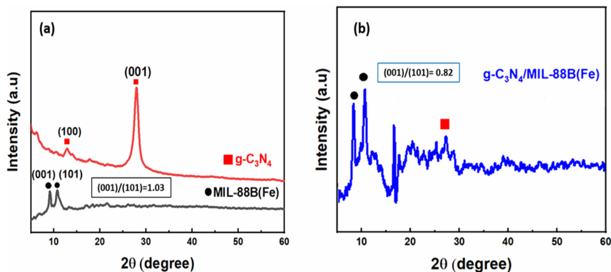
Figure 3. XRD pattern, (a) g-C_3N_4 nanosheets, Metal-Organic framework MIL-88B(Fe), and (b) g-C_3N_4 /MIL-88B(Fe) nanocomposite.
