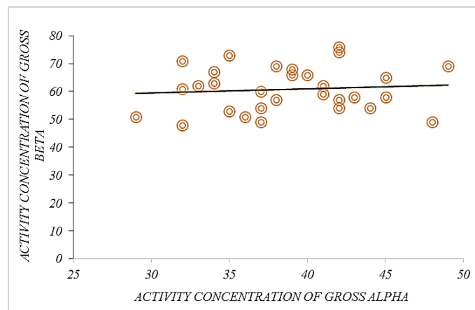
Figure 1. The weak correlation between gross beta and alpha radioactivity concentrations (mBq L -1 ).
