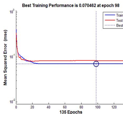
Bayesian Regularization
