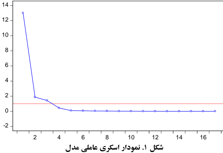
Scree Plot (Ordered Eigenvalues)
