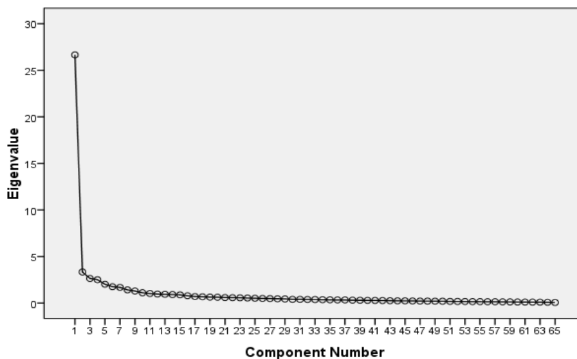
Scree Plot
