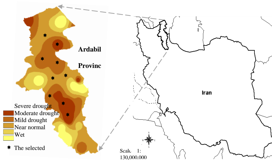
Fig. 1. Drought zoning map of study area and the selected villages
