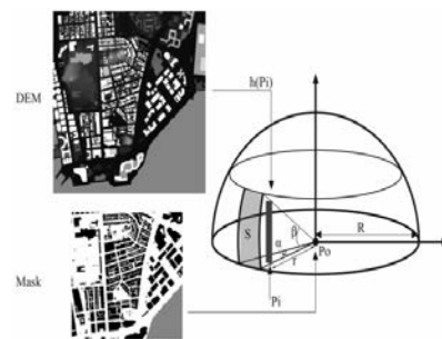
Figure 3. Illustration of the algorithm for calculating SVF. The Mask layer defines the pixels whose SVFs are to be calculated (P i ) and the DEM layer stores height information of the urban surface (h(P i )). \alpha is the rotation angle and R is the searching radius. P i is the pixel with the largest elevation angle \beta along a certain direction. Surface S is the segment of the sky obstructed by P i .
