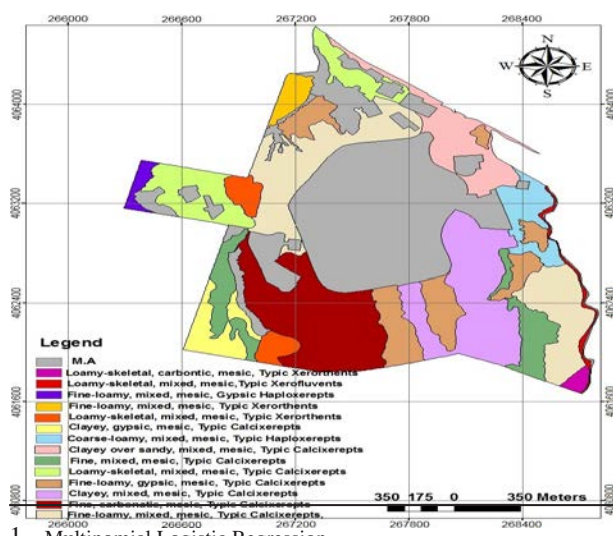
1- Multinomial Logistic Regression
