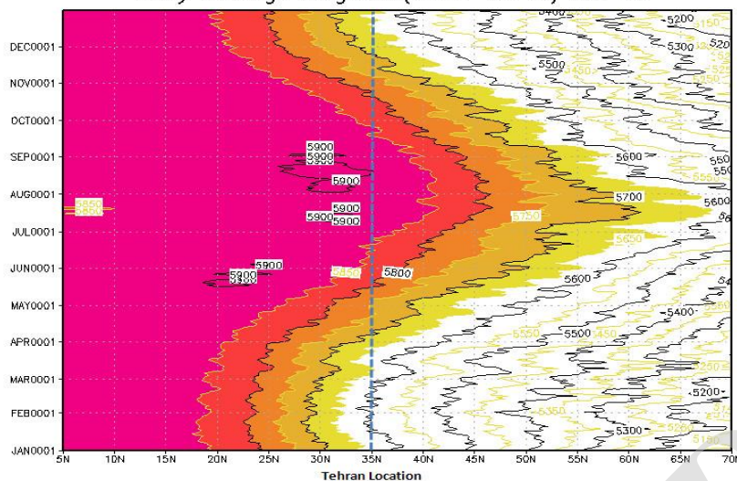
daily 500hgt longterm(1945-2014) lon 50'
