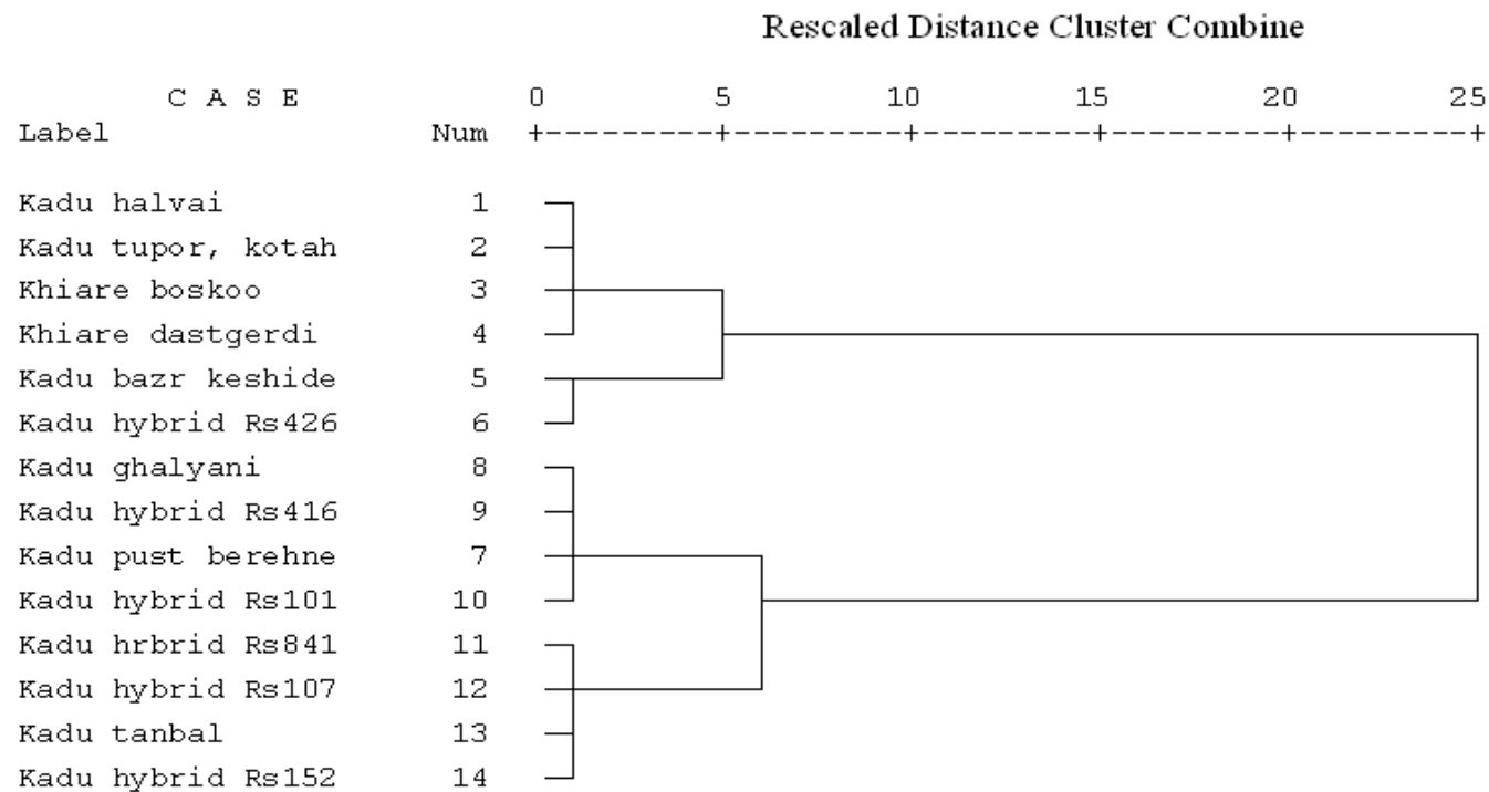
Dendrogram using Average Linkage (Between Groups)
