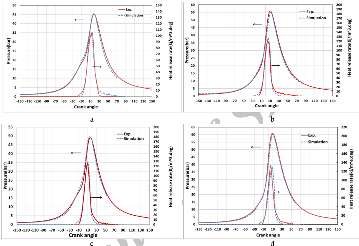
Figure 5- Validation of model results using in-cylinder pressure and heat release rate histories: (a) 1500rpm and spark timing of 19 CAD BTDC (b) 1500rpm and spark timing of 26 CAD BTDC (c) 1200rpm and spark timing of 19 CAD BTDC (d) 1200rpm and spark timing of 26 CAD BTDC
