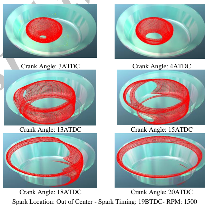
Figure 7- Development of flame front and its collision to the combustion chamber walls when spark plug is located out of center شکل ۷- روند گسترش جبهه شعله و برخورد به دیواره در حالت شمع خارج از مرکز
