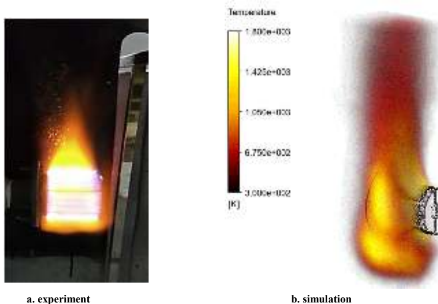
Figure 12- Picture of the fire at 11kW in 0.64 equivalence ratio
