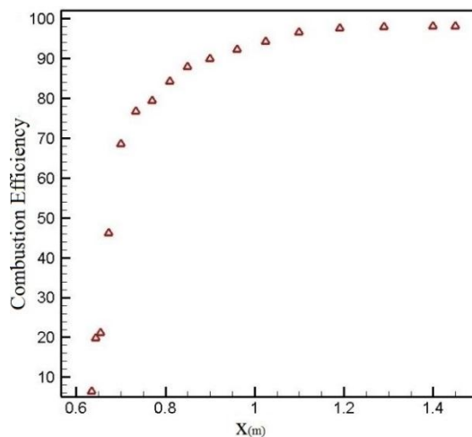
Figure 12- Combustion efficiency for scramjet with quad-cavity and dual-fuel injection
