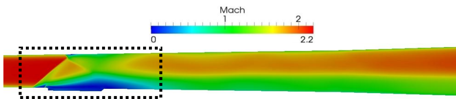
a) Mach number distribution in the supersonic single-cavity combustion chamber
