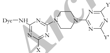
X, Y and Y' = labile atoms or groups
