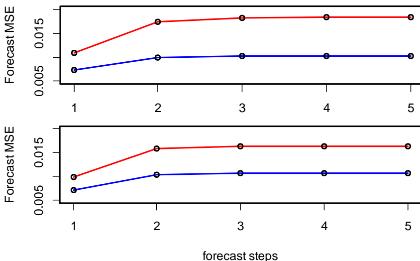
Figure 3: Comparison of forecasts covariances in 5-steps for CMLE estimators — and RSB estimators — (up figure for Golden and down for free Dollar)
