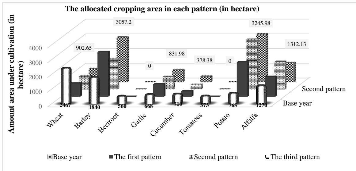
Fig. 2- Compares the current pattern of cropping pattern programming fuzzy goal weight model (equal weights, increasing and decreasing goals)
