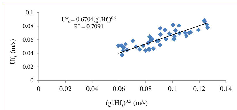
Fig.11- Variations of U_{fs} versus (g'.hfs)^{0.5} in separation point
