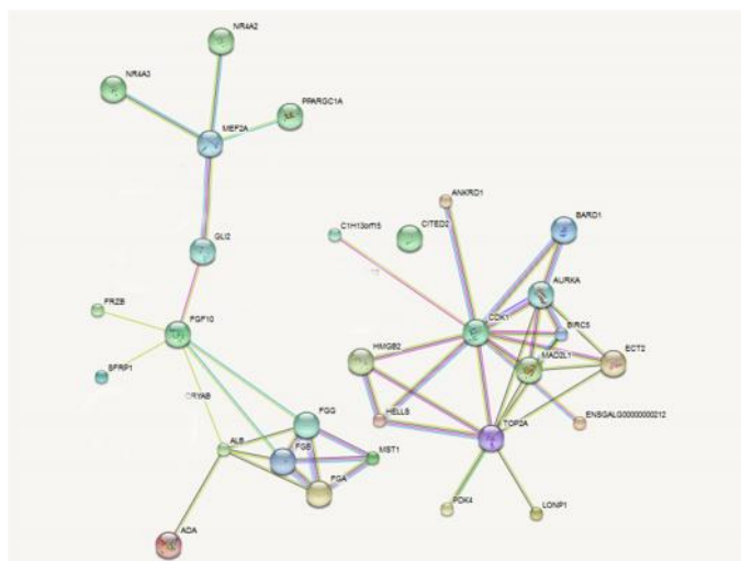
Fig. 2. The Protein-Protein Interaction network for apoptosis pathway genes of Gallus gallus showing gene clusters of ascites sensitive Aryan chickens ( P=0.000076 ). The similar colored nodes are related to a cluster, and larger nodes are proteins whose three-dimensional structures are detected
