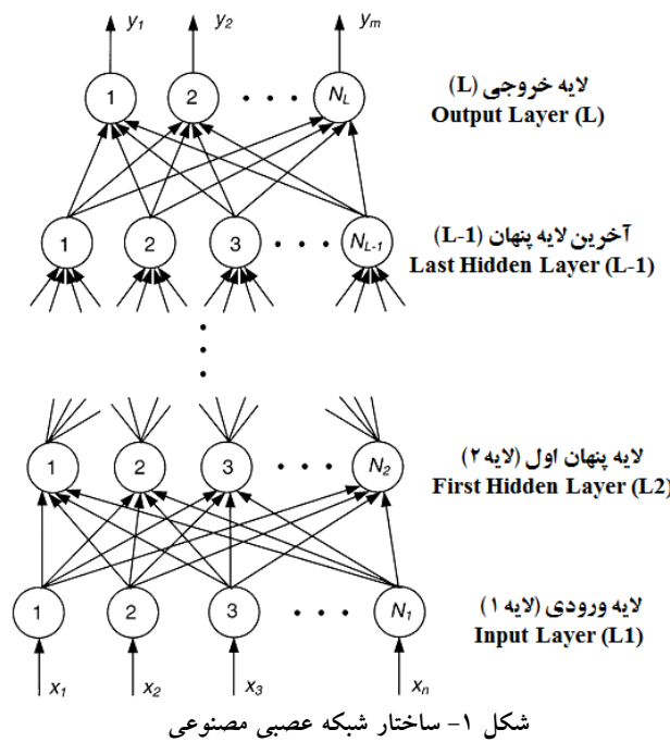
Figure 1. Architecture of Artificial Neural Network
