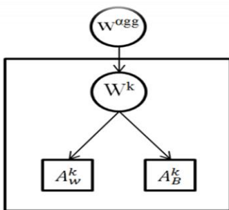
Figure 2. The probabilistic graphical model of the bayesian BWM
