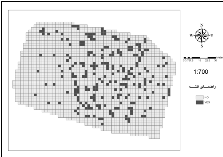
Fig. 2. Sampling plots networks for survey of Lilium ledebourii distribution.
