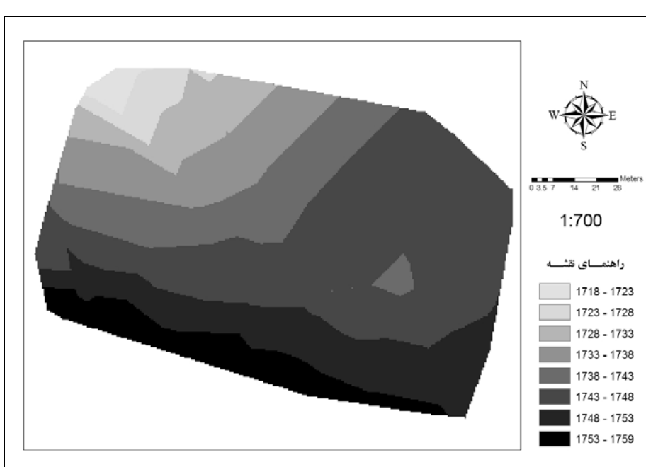
Fig. 1. Digital elevation model of Lilium ledebourii site.
