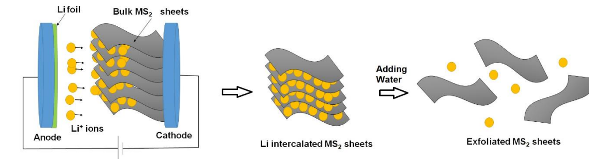
Electrochemical Li intercalation inside battery set up
