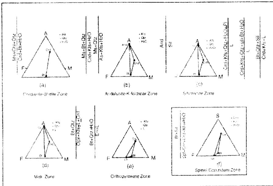
Fig 2 Phase relations and metamorphic reaction for pelitic rocks of the Kalaybar aureole. SFM diagram is used for quartz-bstent rocks.
