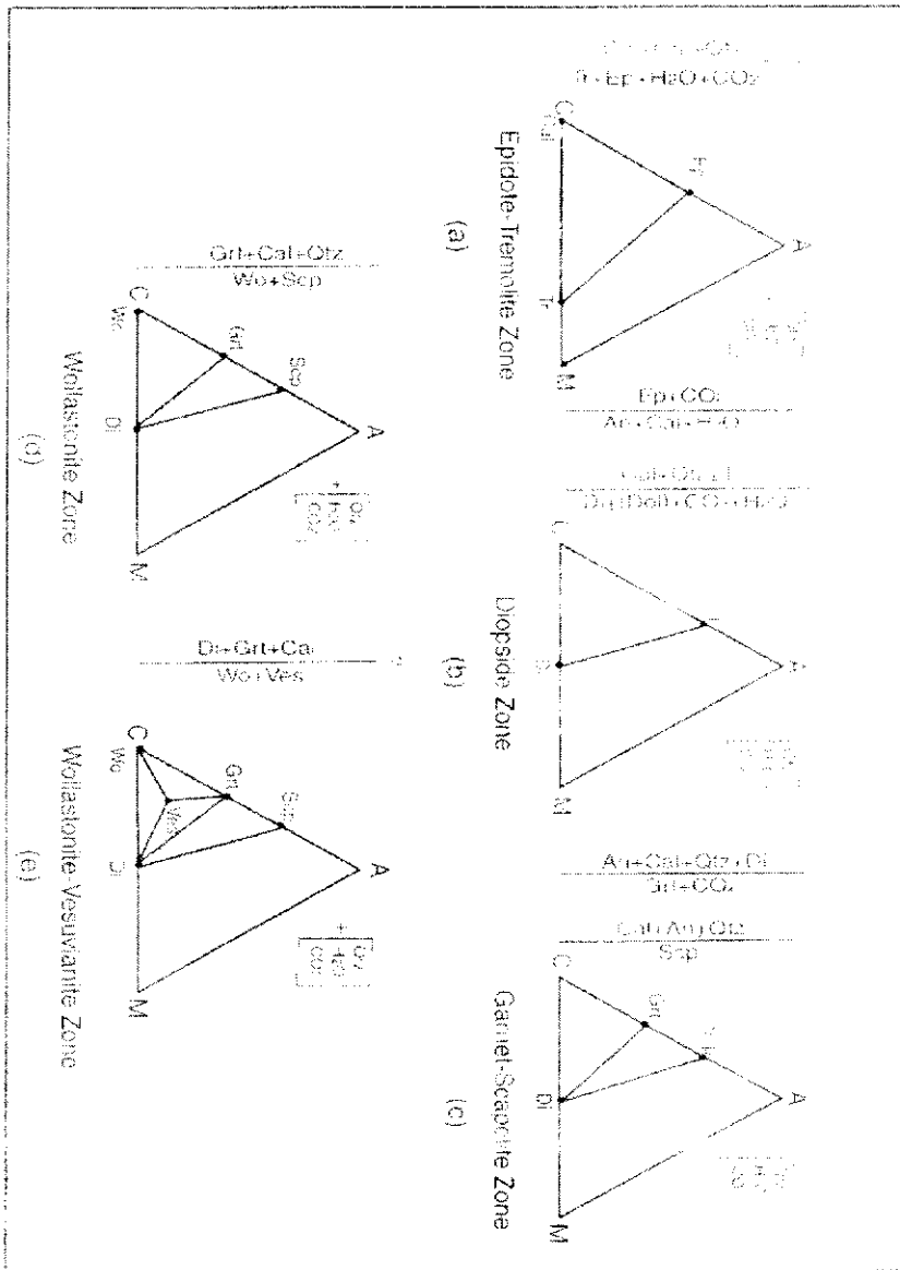
Fig 4 Phase relation and metamorphic reaction for calc-silicates of the Kalaybar aureole.
