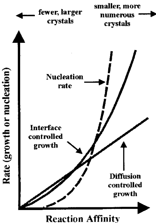
Fig. 1 Schematic plot showing relationship between nucleation and growth rates as function of reaction affinity ( A_r ). A_r is function of amount of overstepping in temperature from equilibrium. For low degree of overstepping, growth rate is much larger than nucleation rate, whilst at higher amount of overstepping nucleation rates are high [3].
